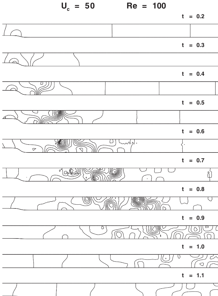
Figure 5. The computed time-varying pressure contours.
