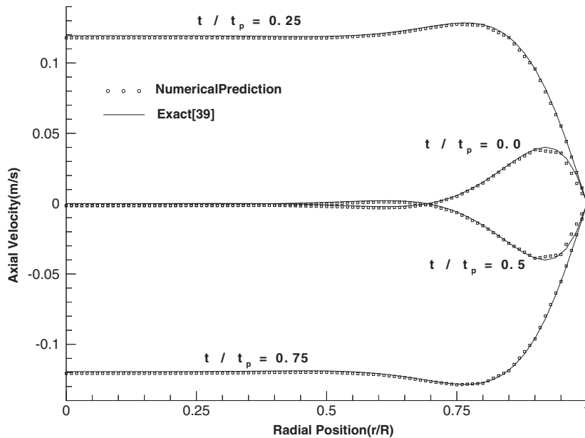
Figure 6. Analytical and predicted axial velocity profiles for transient flow in a compliant tube.
