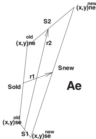
Figure 2. Schematic of the notations given in Equation (28).
