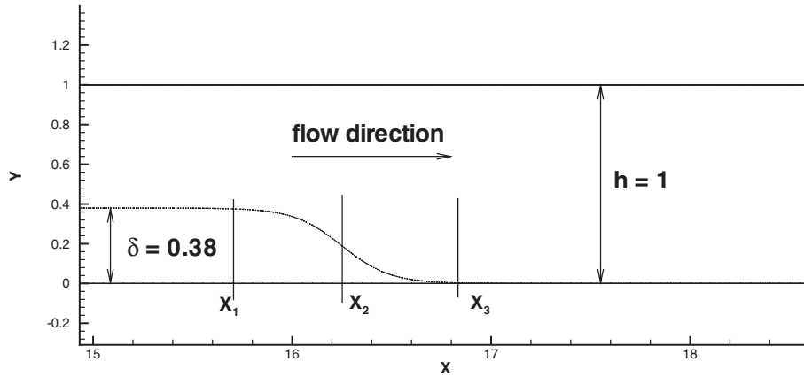
Figure 3. Schematic of the indented wall.
