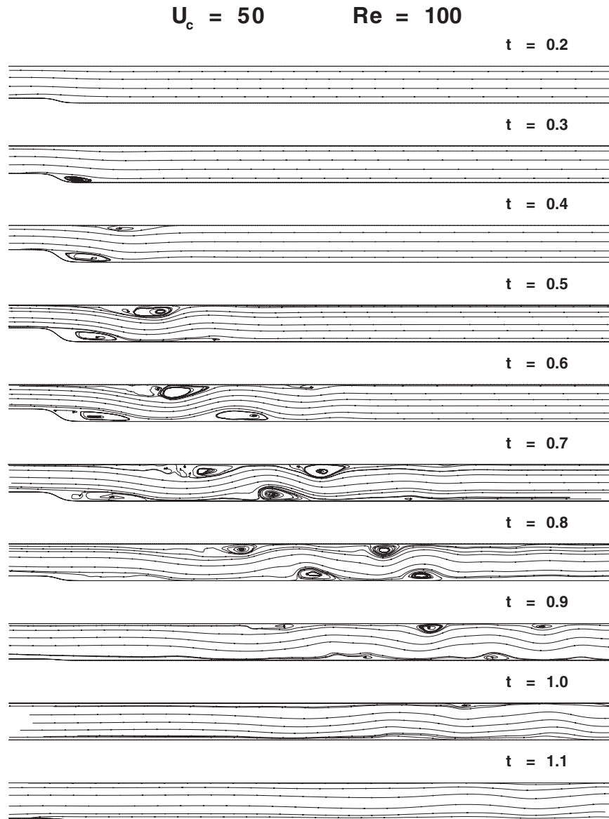
Figure 4. The computed time-varying streamlines.
